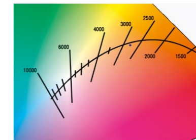
CIE DIAGRAM
